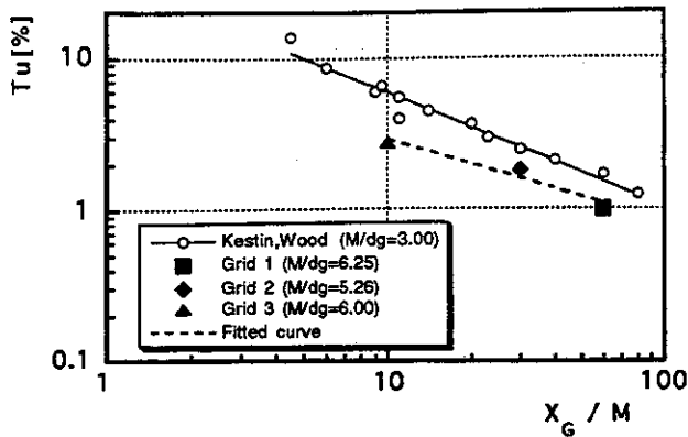
(a) The decay of free stream-turbulence
