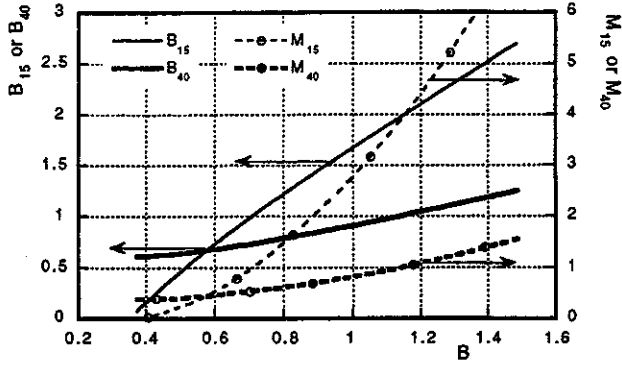
Figure 4 Relationship of local and mean blowing ratio
