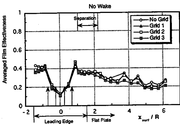
Figure 14 Averaged film effectiveness without the wake effect ( B=0.8 )
