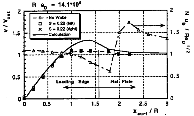
Figure 5 Velocity and heat transfer distribution around the leading edge
