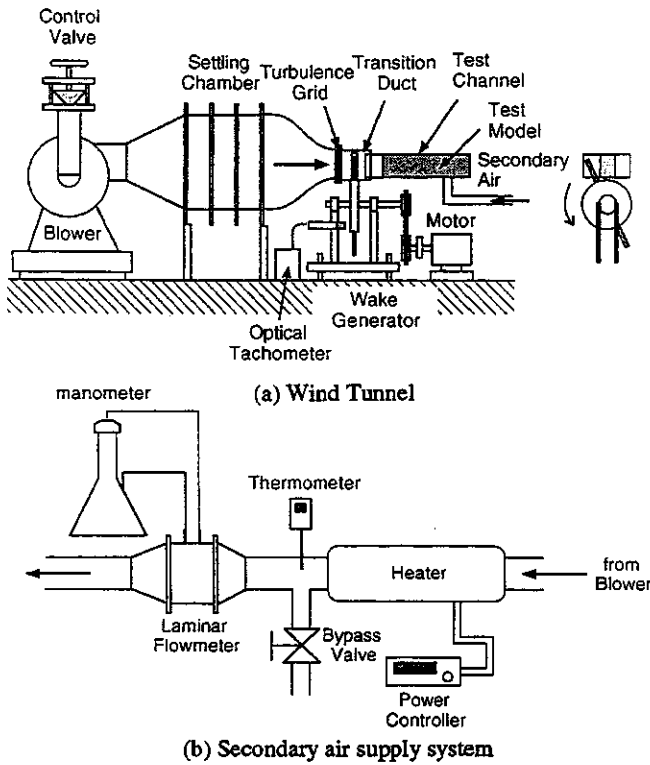
Figure 1 Schematic layout of the test apparatus
