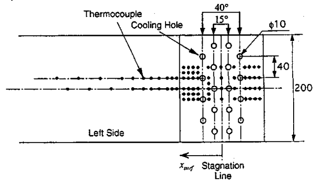
Figure 3 Layout of thermocouples and film holes (Unfolded surface view)
