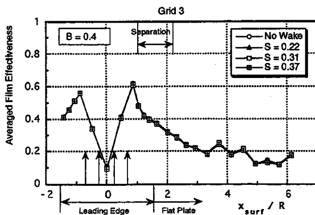
Figure 18 Averaged film effectiveness with wake and free-stream turbulence effect ( B=0.4 , Grid3)
