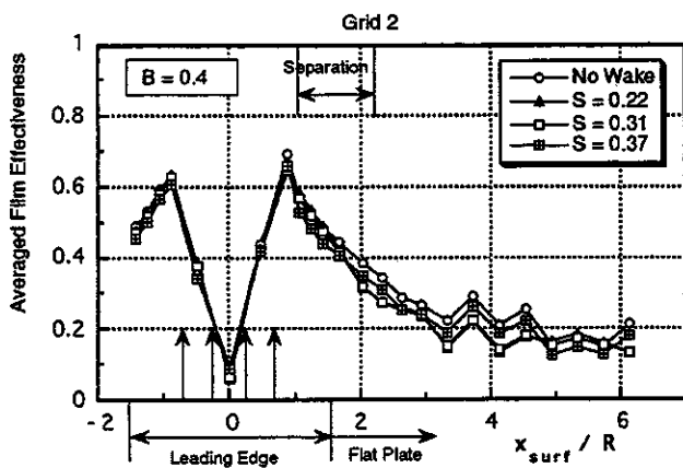
Figure 17 Averaged film effectiveness with wake and free-stream turbulence effect ( B=0.4 , Grid2)
