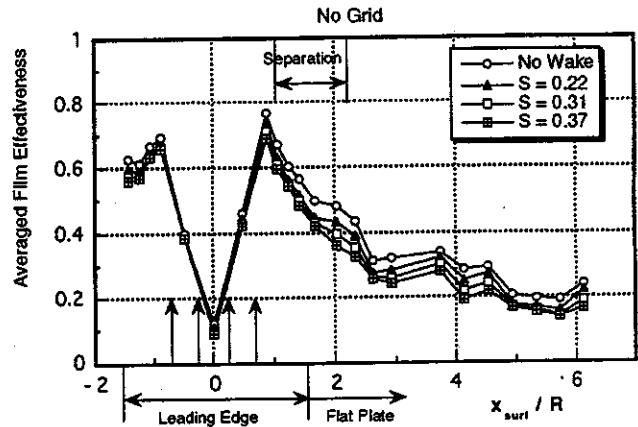
Figure 8 Averaged film effectiveness without the turbulence grid ( B=0.4 )
