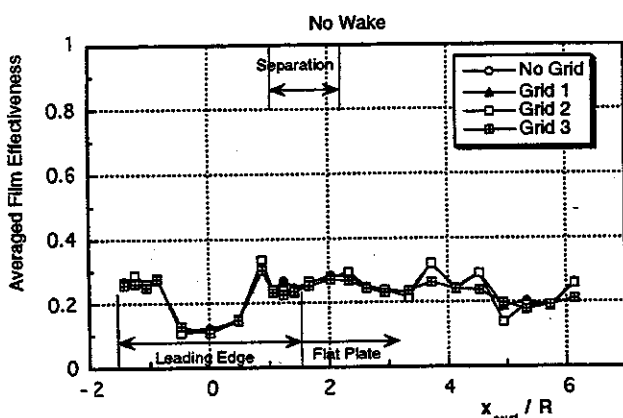
Figure 15 Averaged film effectiveness without the wake effect ( B=1.2 )
