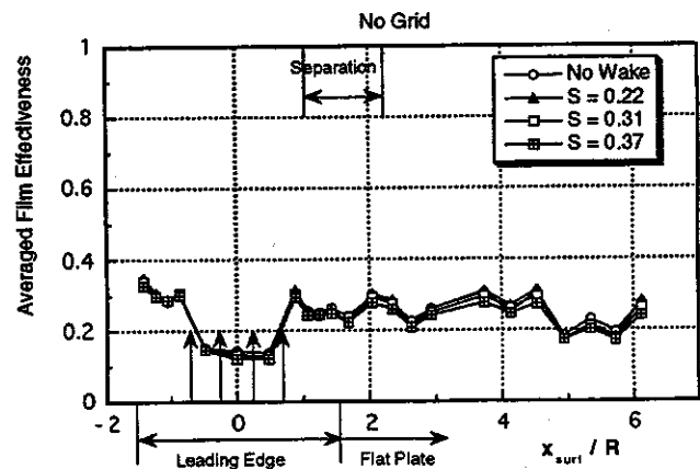
Figure 10 Averaged film effectiveness without the turbulence grid ( B=1.2 )
