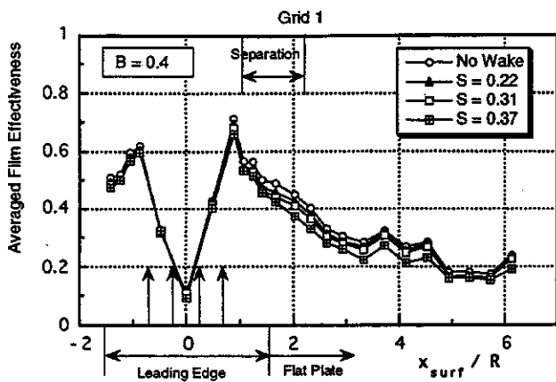
Figure 16 Averaged film effectiveness with wake and free-stream turbulence effect ( B=0.4 , Grid1)
