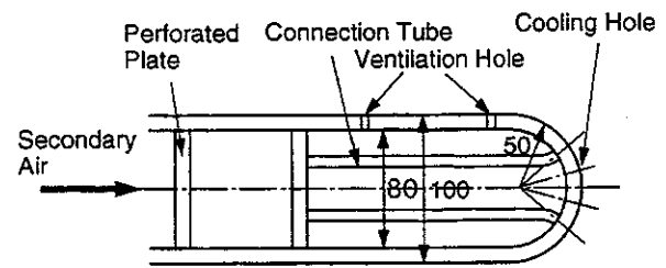
Figure 2 Test model
