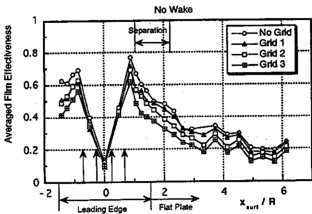
Figure 13 Averaged film effectiveness without the wake effect ( B=0.4 )
