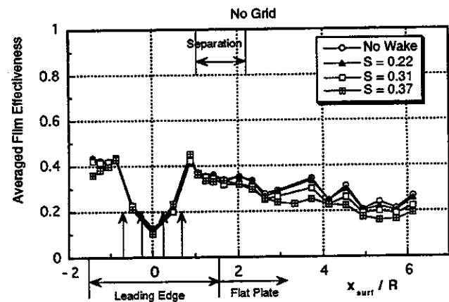
Figure 9 Averaged film effectiveness without the turbulence grid ( B=0.8 )
